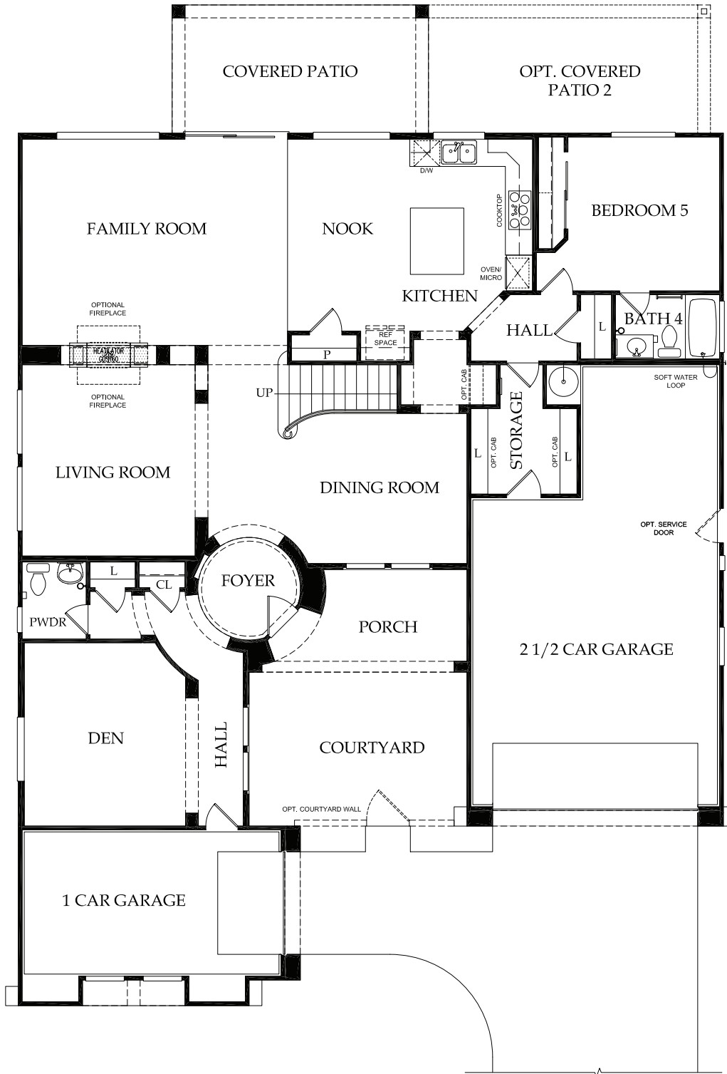
ELEVATION 'A' First Floor Plan
